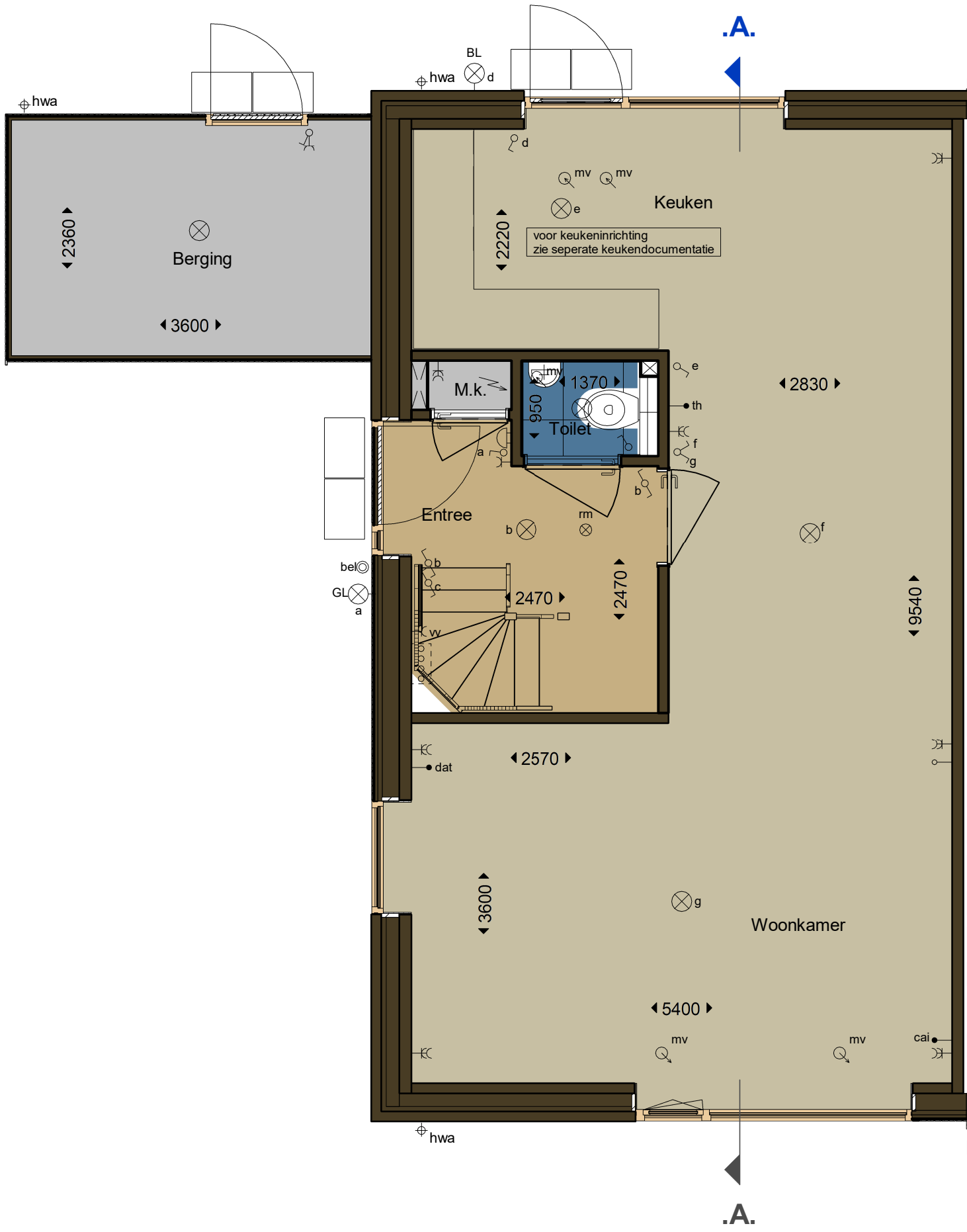
Type A Bnr. 2/4/6/8/10/12/14/16/18/20 begane grond 1:50
